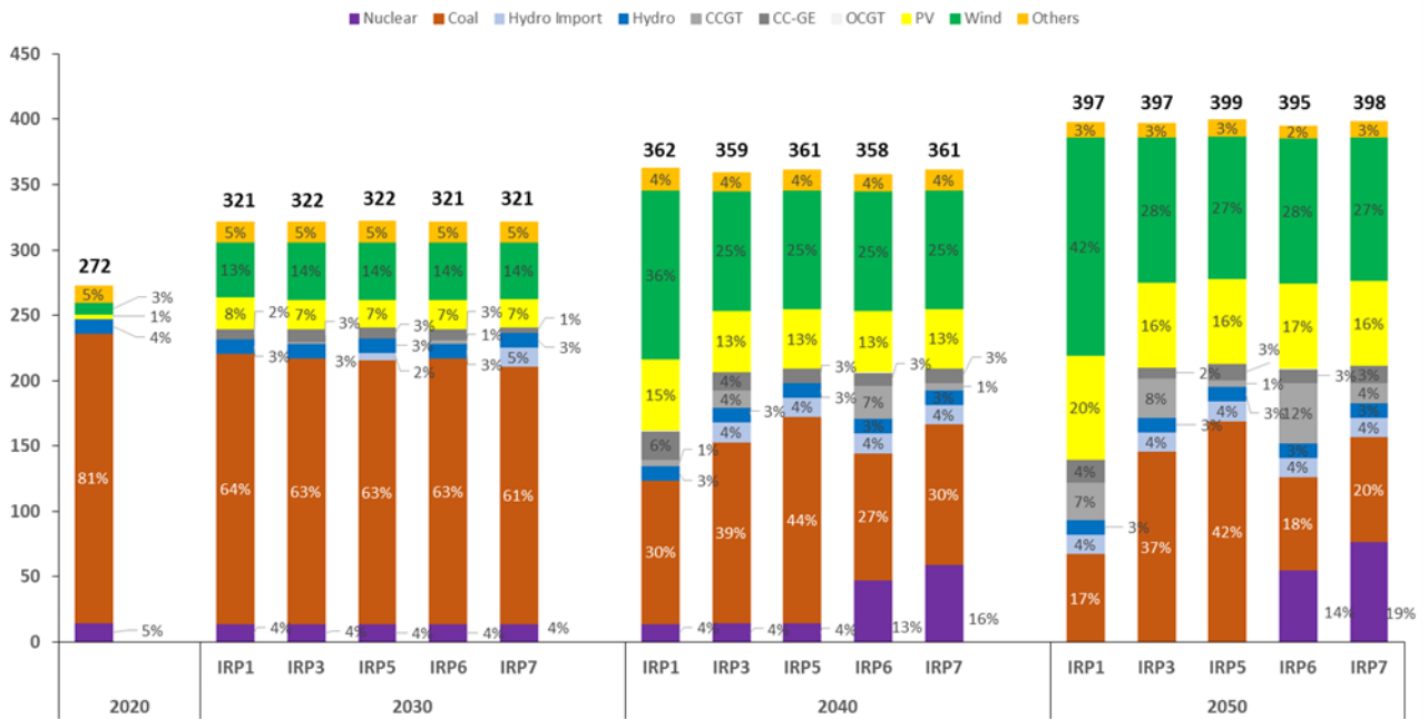
Figure 18: Consumed Energy (TWh) for the No RE Annual Build Rate (IRP1), Median-growth (IRP3), Market-linked Gas Price (IRP5), Carbon Budget (IRP6) and Carbon Budget plus Market-linked Gas Price (IRP7) Scenarios
