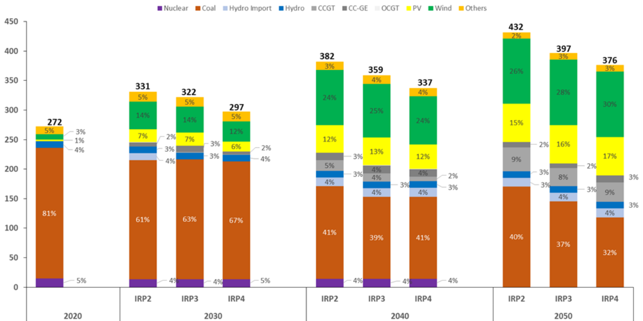
Figure 16: Consumed Energy (TWh) for the High- (IRP2), Median- (IRP3) and Low-growth (IRP4) Scenarios
