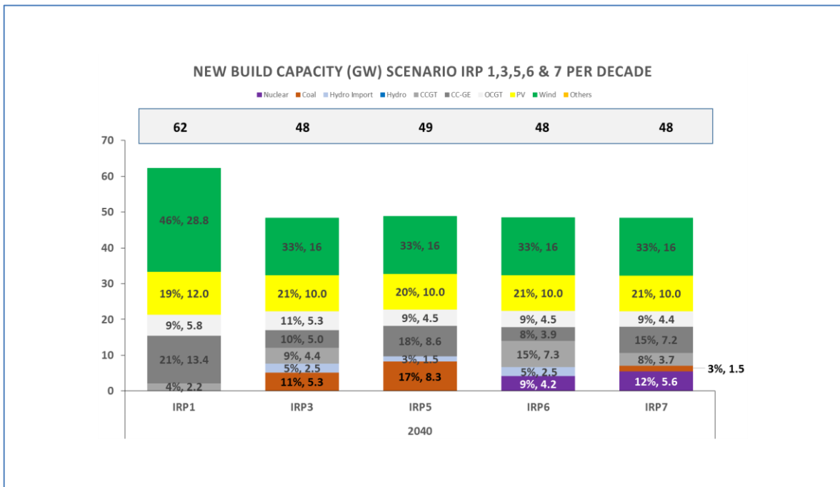
Figure 24: New Build Capacity for the Period 2031–2040
